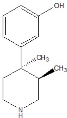
(+)-(3R,4R)-3-(3,4-Dimethyl-4-piperidinyl)phenol
